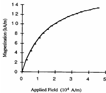
Fig. 1. Magnetization as a function of applied field.
